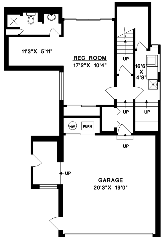
LOWER FLOOR
